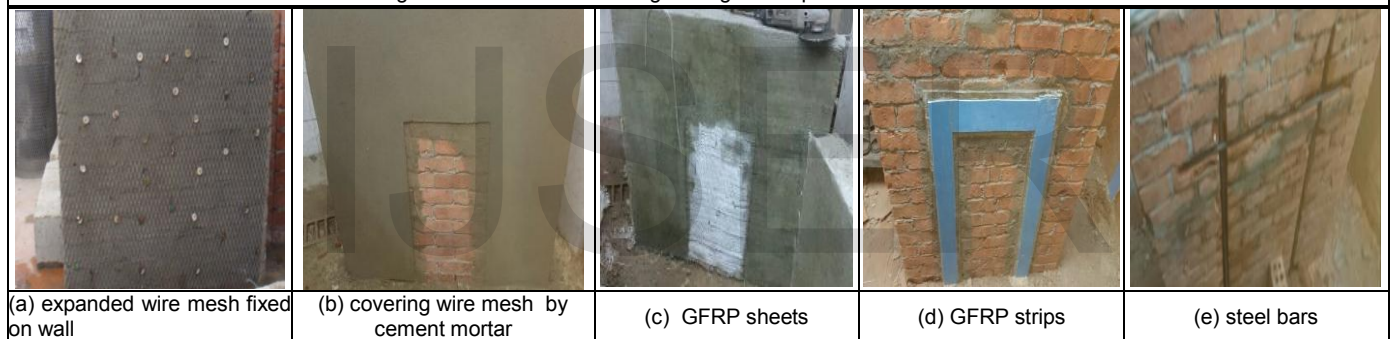
Fig. 3. Walls specimens strengthened using the suggested schemes
