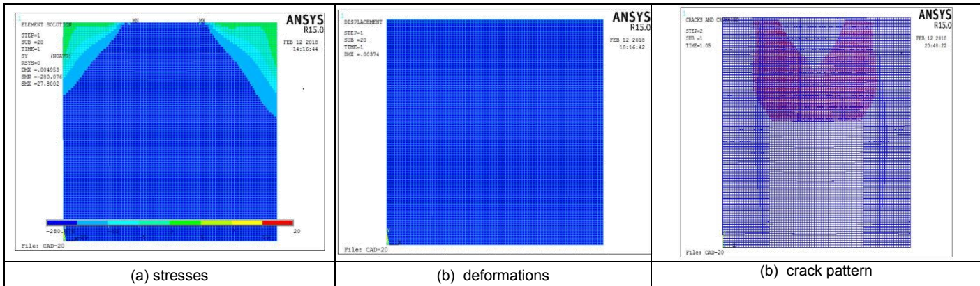
Fig. 21 The strengthened wall under service loads – before making the opening
