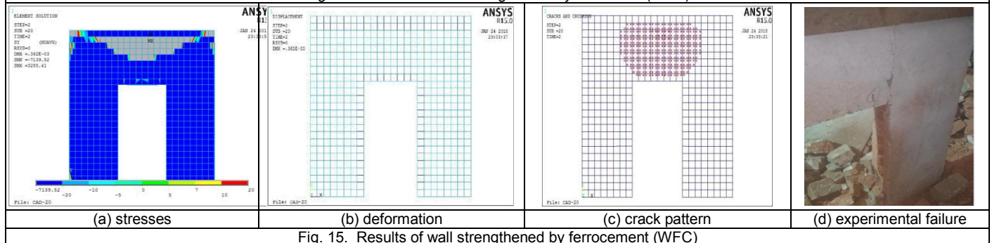
Fig. 15. Results of wall strengthened by ferrocement (WFC)
